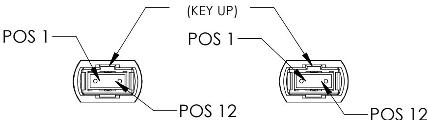
MTP CONNECTOR END VIEW SEE NOTE 3, SCALE 3:2
